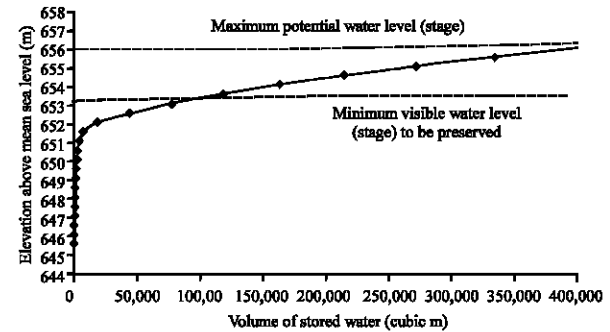
Fig. 7: Stage-volume cure for Al-alb Dam, Riyadh, Saudi Arabia
