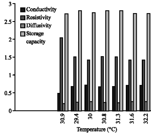
Fig. 9: Comparison of temperature with thermal conductivity, resistivity and diffusivity and storage capacity of concrete sample A6 (mixture 1:4.3:4.0)
