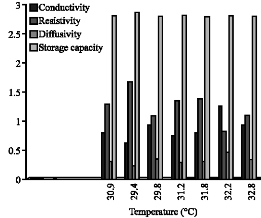
Fig. 8: Comparison of temperature with thermal conductivity, resistivity and diffusivity and storage capacity of concrete sample A5 (mixture 1:3.1:3.0)
