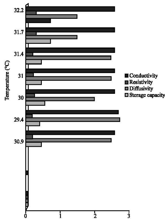
Fig. 10: Comparison of temprature with thermal conductivity, resistivity and diffusivity and storage capacity concreete sample A7 (mixture 1:5.6:5.0)
