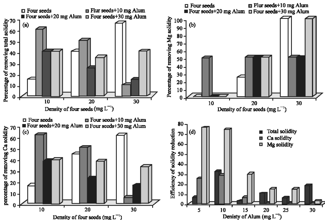
Fig. 3: (a-d) Efficiency of solididity reduction
