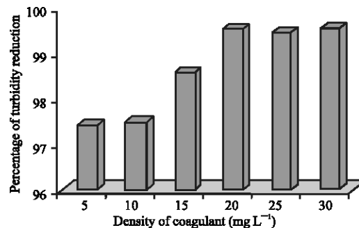
Fig. 1: Percentage of turbidity reduction by Alum
