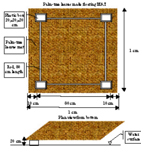
Fig. 1: Details for palm leaf mat used for evaporation reduction
