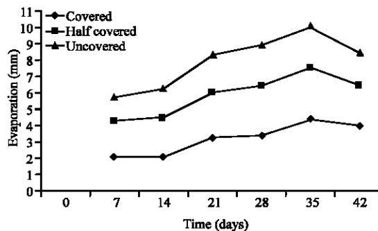
Fig. 3: Evaporation records from the three pools
