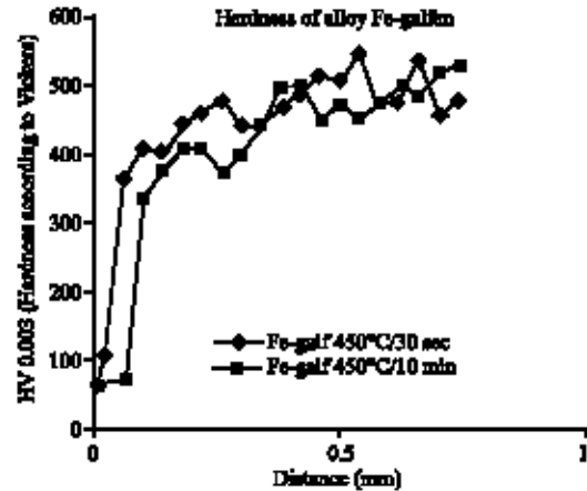
Fig. 6: Hardness of galvanized steel samples ( T_g = 450^\circ\text{C} , t_g = 30 sec and t_g = 10 min)
