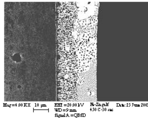
Fig. 4: The points of measurements with EDS in galvanized steel sample 450^\circ\text{C} , 30 sec
