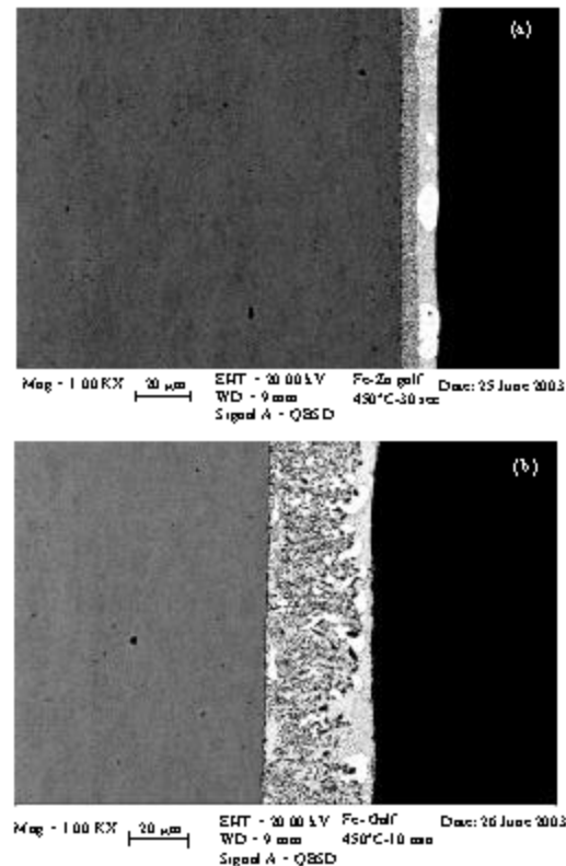
Fig. 2: Microstructure of galfanized steel samples, a: 450°C, t_d = 30 sec picture and b: 450°C, t_d = 10 min
