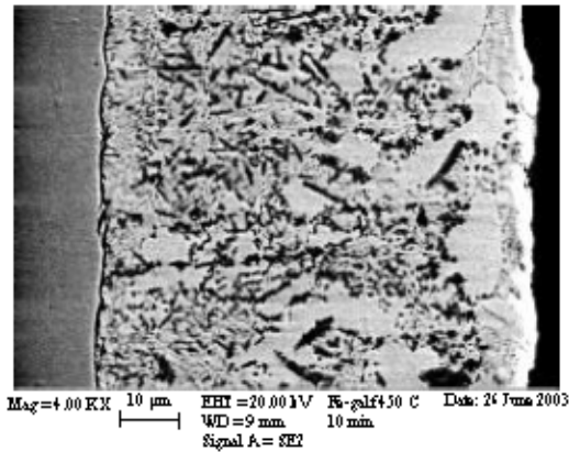
Fig. 3: Microstructure of galvanized steel samples in T_g = 450^\circ\text{C} and t_g = 10 min
