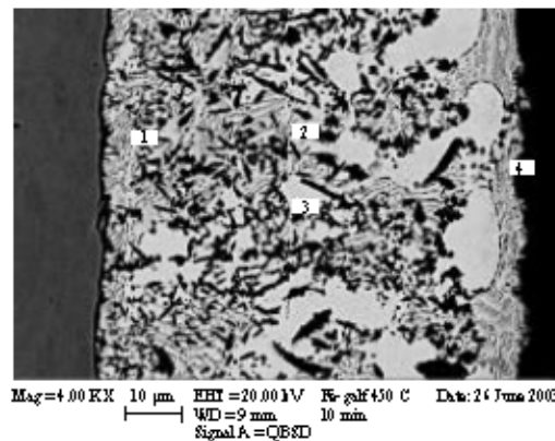
Fig. 5: The points of measurements with EDS in galvanized steel sample 450^\circ\text{C} , 10 min
