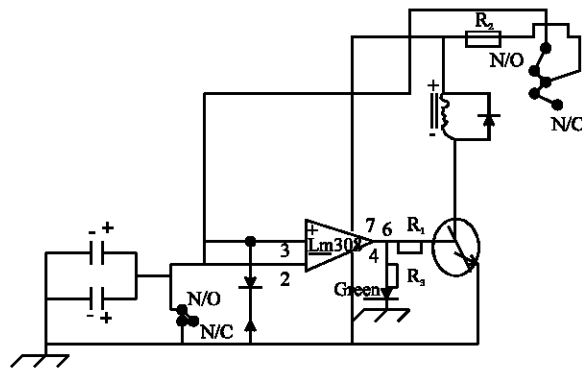
Fig. 3: Charging unit
