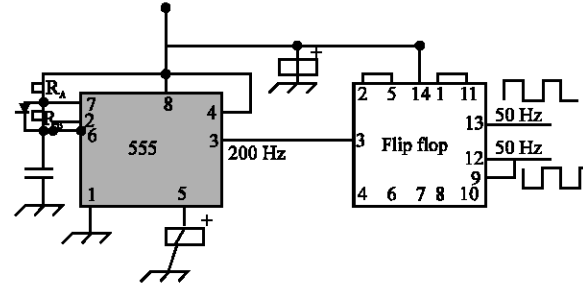
Fig. 4: Pulse generator unit
