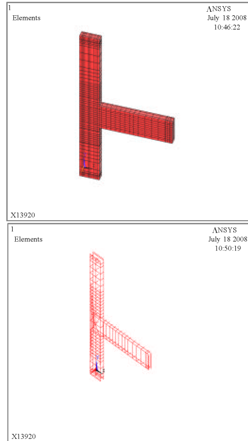
Fig. 4: Modeling details in ANSYS
