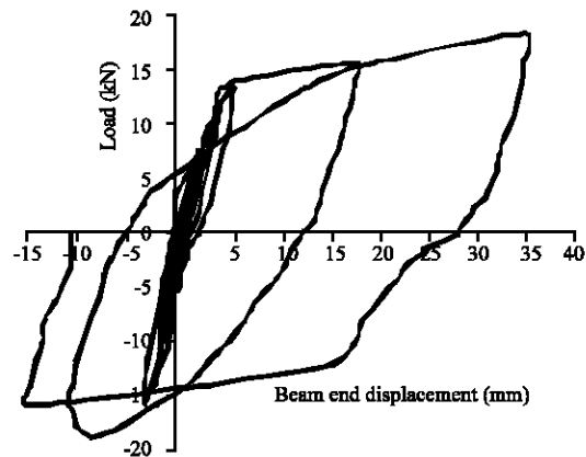
Fig. 10: Load-displacement curve of B2-13920
