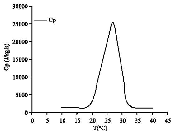
Fig. 2: Specific heat capacity of gypsum/pcm (Maha et al. , 2006)
