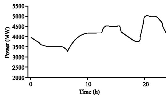
Fig. 1: Daily national electric consumption (SONELGAZ) Algeria August 2005)
