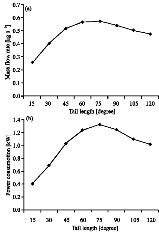
Fig. 10: Effects of tail angles on (a) mass flow rates and (b) power consumption
