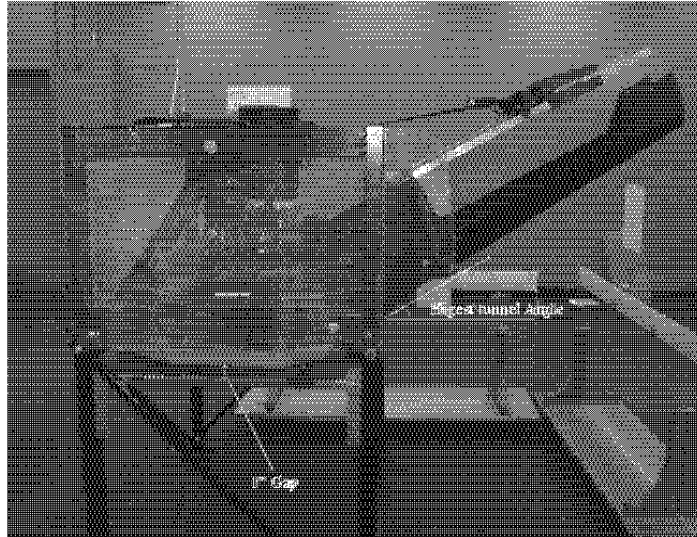
Fig. 12: Test rig setup without a collector
