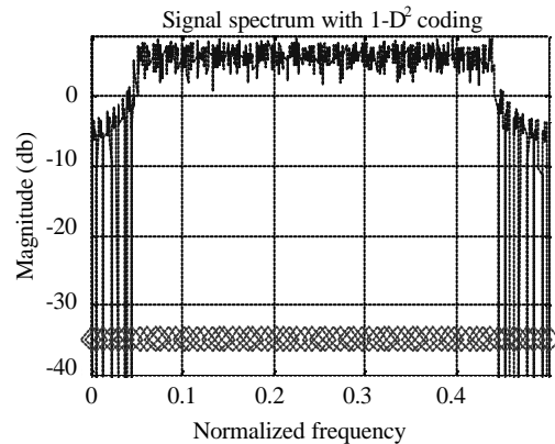
Fig. 4: Spectrum of OFDM using 1-D 2 coding
