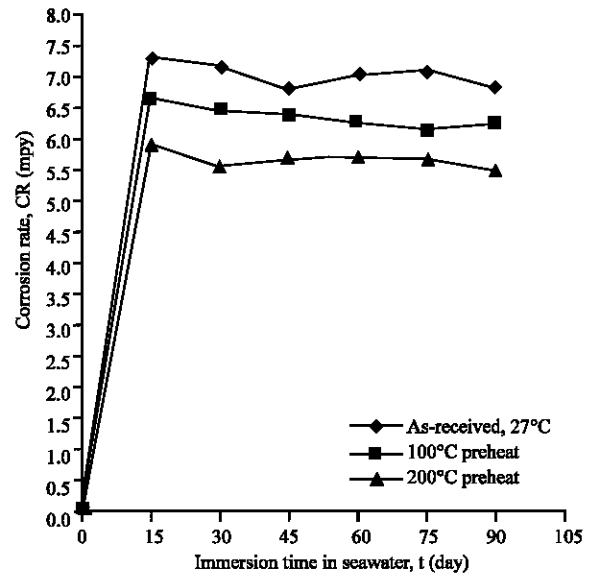
Fig. 6: Plot of corrosion rate of single-pass pipe weldment with immersion time in seawater
