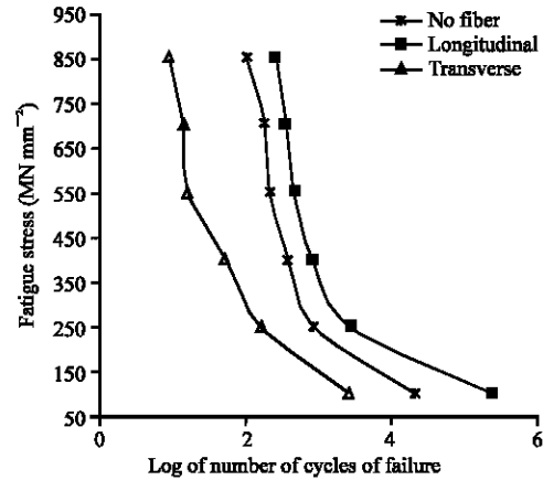
Fig. 4: Plot of fatigue stress vs log of number-of-cycles to failure
