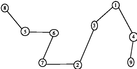
Fig. 3: Chromosome B
