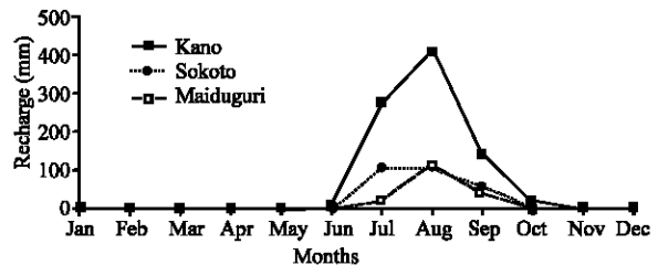
Fig. 5: Comparison of average recharge for 2001-2003
