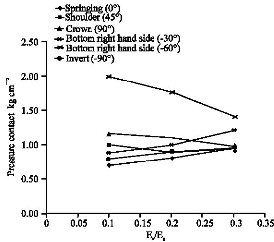
Fig. 8: Pressure contact distribution for various E_s/E_g
