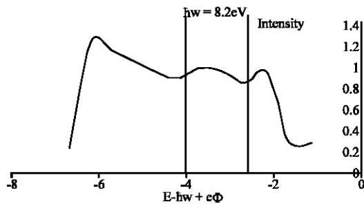
Fig. 12: Experimental EDC measured at h\nu = 8.2\text{eV}
