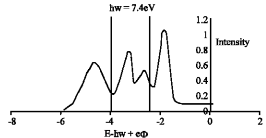
Fig. 3: Theoretical EDC measured at \hbar\omega = 7.4\text{eV}
