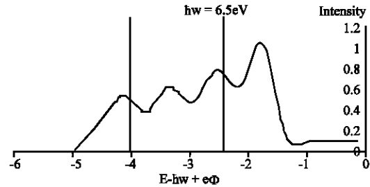
Fig. 1: Theoretical EDC measured at \hbar\omega = 6.5\text{eV}
