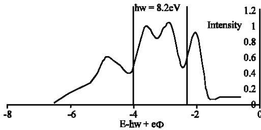
Fig. 6: Theoretical EDC measured at h\nu = 8.2\text{eV}
