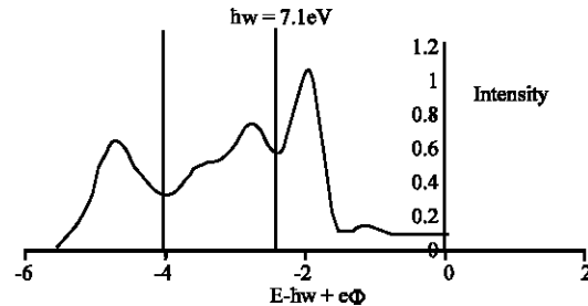
Fig. 2: Theoretical EDC measured at \hbar\omega = 7.1\text{eV}
