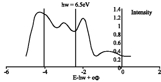
Fig. 7: Experimental EDC measured at h\nu = 6.5\text{eV}
