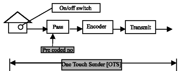
Fig. 1: One Touch Sender [ OTS ] block diagram
