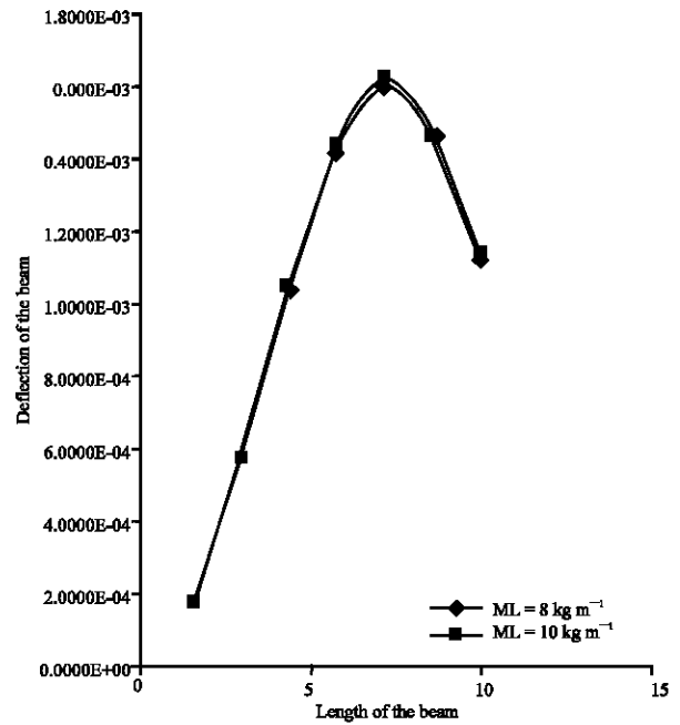
Fig. 5: The prestressed Rayleigh beam to a moving mass at \varepsilon = 0.1m , t = 0.5s , at various values
