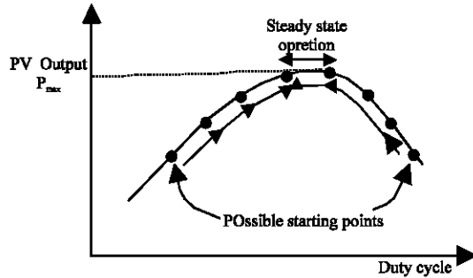
Fig. 8: MPPT tracking process
