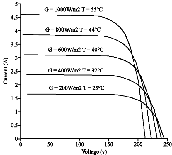
Fig. 3: I-V characteristics of PV generator
