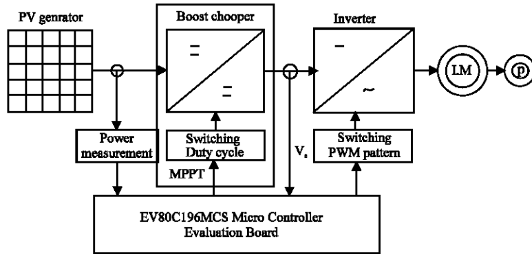
Fig. 1: Block diagram of PV pumping system
