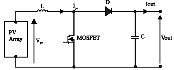
Fig. 5: Step-up chopper
