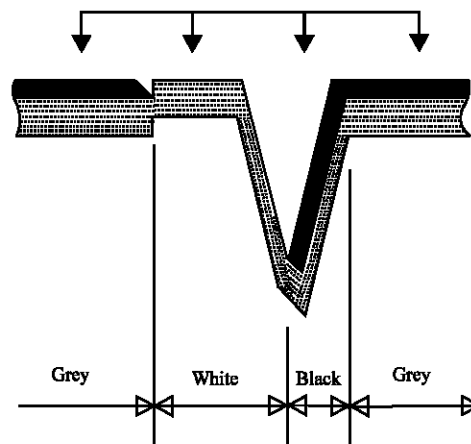
Fig. 5: Contrast shade sequence of a microcrack
