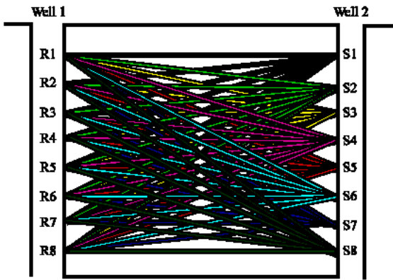
Fig. 2: Seismic data crosswell geometry
