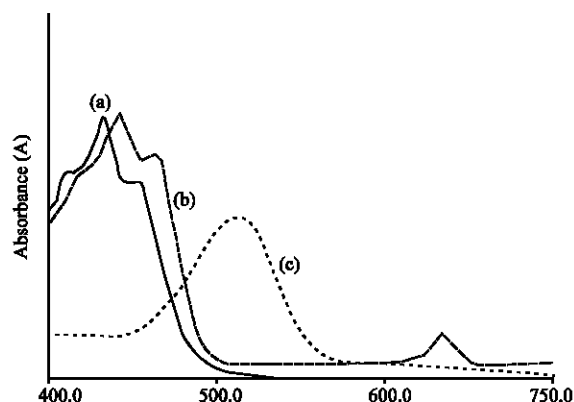
Fig. 1: Electronic absorption spectra patterns of the ornamental horticulture flowers in various solvent, (a) Allamanda, Broom weed, Pride of Barbados (ethanol); water leaf (chloroform); Bushmarigold (diethyl ether); Gloriosa (lime water) and sunflower (acetone), (b) Allamanda, Bouhinia, Bouganvillea (acetic acid); Bushmarigold (diethyl ether), Gloriosa (phenol) and pride of barbados (ethanol). (c) Bouhinia, Sunflower (ethanol); Bouganvillea (water and phenol); broom weed (acetone); crotalaria (acetone and phenol; Glorisa; pride of barbados acetic acid). Hibiscus (ethanol and phenol); Hibiscus sobdoriffa (water leaf (phenol)
