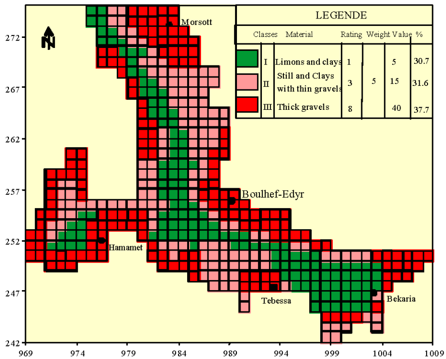
Fig. 4: Vulnerability map related to unsaturated zone
