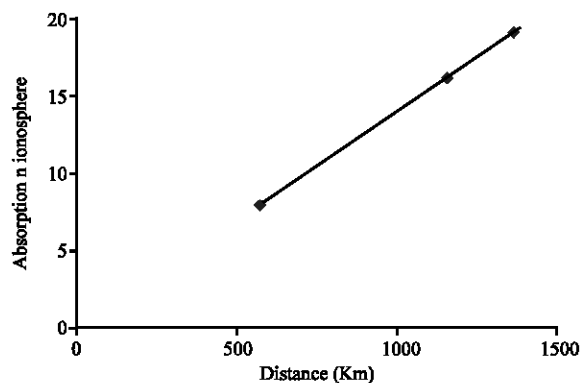
Fig. 2: Ionospheric absorption variation with distance
