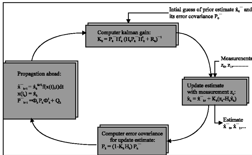
Fig. 1: Attitude determination loop
