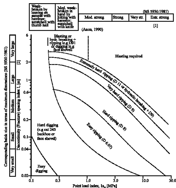
Fig. 4: Revised excavability graph (Pettifer and Fookes, 1994)
