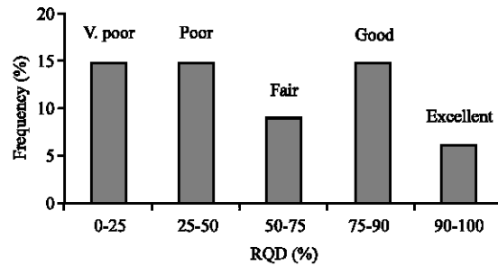
Fig. 1: Percentage distribution of RQD values of sandstone in Sennar PHP site
