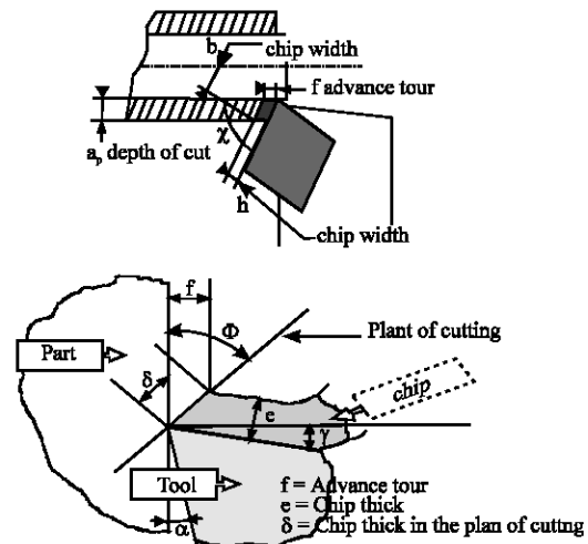
Fig. 2: Diagram of orthogonal continuous cutting
