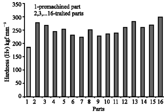
Fig. 4: Evolution of ball burnished superficial hardness (Hv)
