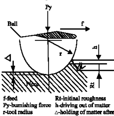
Fig. 2: Treatment by superficial plastic deformation
