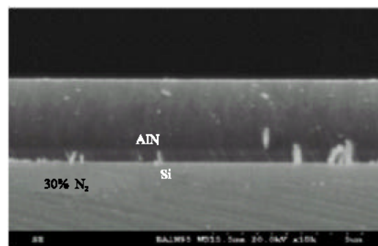
Fig. 4: SEM cross section image at 30% N_2 concentration
