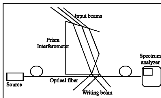
Fig. 6: A schematic of the prism wavefront-splitting interferometer
