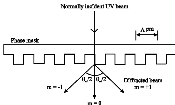
Fig. 12: Schematic of the UV radiation at normal incidence of a phase masks
