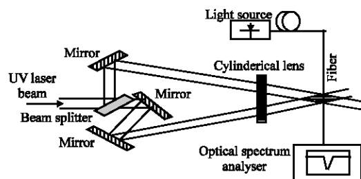
Fig. 3: Amplitude-splitting interferometer
