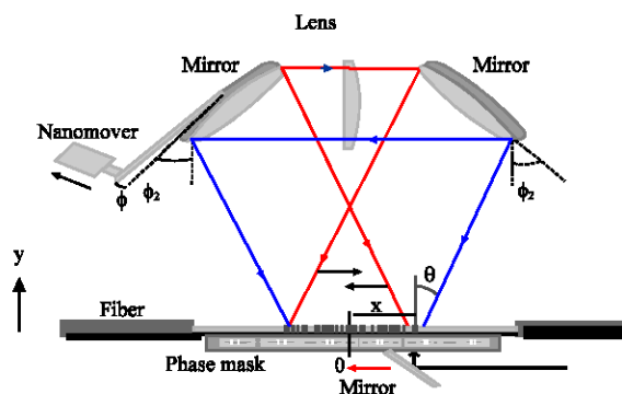
Fig. 7: Sagnac interferometric phase mask technique
