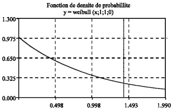
Fig. 4: Weibull's model
