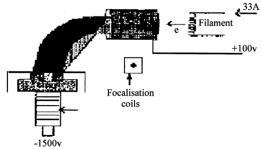
Fig. 2a: DC triode co-sputtering configuration
