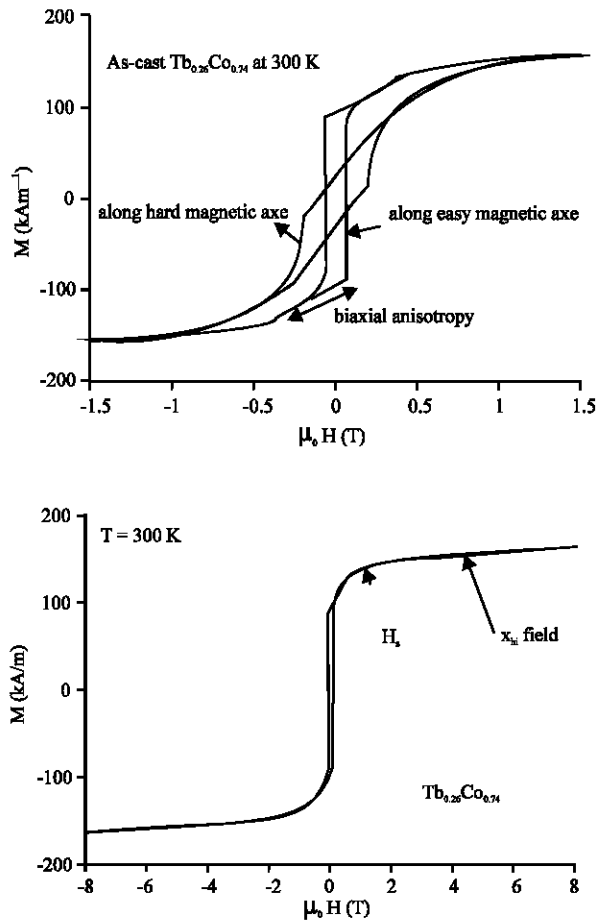
Fig. 3: Magnetisation loops at 300 K for Tb_{0.26}Co_{0.74} in 2 directions. Insert: High field magnetization up to 8 Tesla
