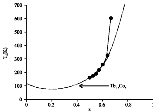
Fig. 1: Curie temperature for a- Tb_{1-x}Co_x as a function of the composition x
