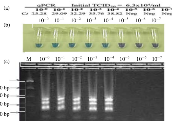
Fig. 11(a-c): Limit of detection (LOD) of SPV-HELD by LAMP and qPCR. SPV-HELD ( TCID_{50} = 6.3 \times 10^4 \text{ mL}^{-1} ) and used as the template for amplification by qPCR (a) and LAMP (b and c). Threshold cycle crossing values for qPCR are indicated (CT). LAMP was analyzed by color change using HNB (b) as well as by agarose gel electrophoresis (c) [49]
