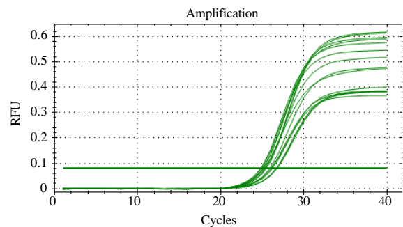
Fig. 1: TLR4 gene RT-qPCR amplification curves
