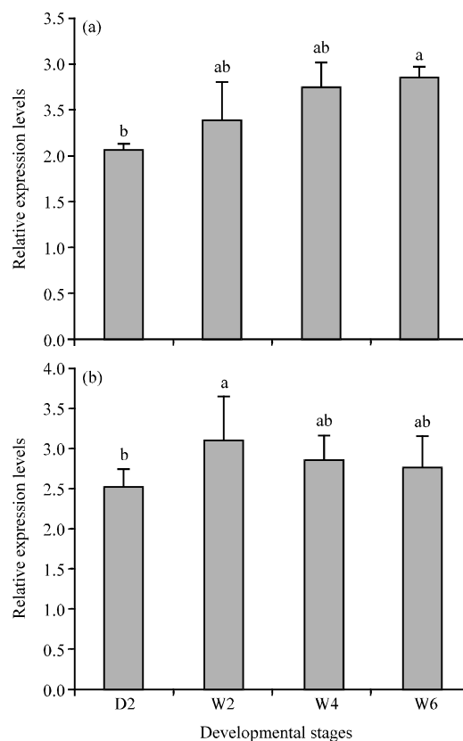
Fig. 5: Relative expression levels (means) of Pekin duck IGF-1 gene. The relative expression levels headed by the same letter denote no significant difference ( p>0.05 ) and headed different letter denote significant difference ( p<0.05 ); D2, W2, W4 and W6 represent the relative expression levels of; a) IGF-1 in breast and b) leg muscle at the 2nd day, the 2nd, 4th and 6th weeks, respectively
