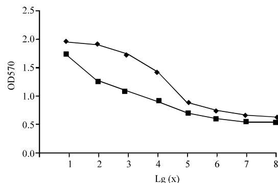
Fig. 4: Protection effect of hIFN- \alpha 1 standard and yak IFN- \alpha 1 on BHK cell. Antiviral activity of the yak IFN- \alpha 1 protein from BHK cells was incubated in the presence of the indicated dilutions of yak IFN- \alpha 1 for 24 h and subsequently infected with VSV. The cells were incubated 20 h following infection and CPE was determined by staining the cells and measuring the absorbance at 570 nm. Symbols are as follows: hIFN- \alpha 1 (■), yak IFN- \alpha 1 (◆) x represent sample dilution folds. Two similar curve both human IFN- \alpha 1 and yak IFN- \alpha 1 protein were drawn according to log (x) value as x-axis and OD570 value in different dilution folds as y-axis. Researchers draw a equation y = -0.3342x + 2.646 ( R^2 = 0.938 ) by linear fitting according to the four point near the value of standard human IFN- \alpha 1 ED50 and draw a other equation y = -0.1808x + 1.626 ( R^2 = 0.9982 ) according to the four point near the value of yak IFN- \alpha 1 ED50. The bioactivity was calculated according to the date supplied with equation
