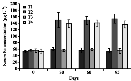
Fig. 2: Serum selenium concentration ( \mu\text{g L}^{-1} ) in goats fed different dietary treatments; T1: [control, basal diet without supplementation (background only)]; T2: basal diet + 0.6 mg Se \text{kg}^{-1} DM; T3: basal diet + 0.6 mg I \text{kg}^{-1} DM; T4: basal diet + (0.6 mg Se \text{kg}^{-1} DM + 0.6 mg I \text{kg}^{-1} DM); the significant differences in serum Se concentration were observed at day 30 of the feeding trial. However, there is no further increase in serum Se concentrations at day 60 and 95 of the experiment
