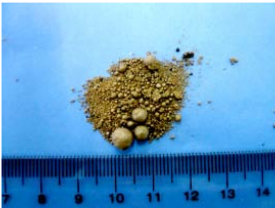
Fig. 1: Bladder stones from four sheep with urinary tract blockage showing the size and surface character similar to potassium magnesium phosphate ( \text{KmgPO}_4.6\text{H}_2\text{O} ) and ammonium magnesium phosphat ( \text{NH}_4\text{MgPO}_4.6\text{H}_2\text{O} ) in crystals structure
