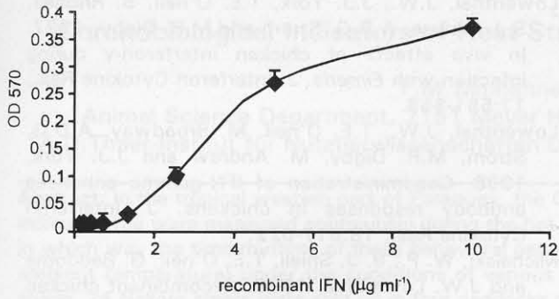
Fig. 4: Functional activity of recombinant turkey IFN- \gamma protein.
