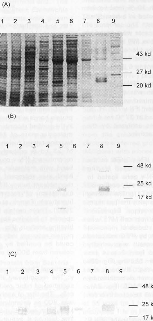
Fig.2: Induction of interferon gamma (IFN- \gamma ) fusion protein expression by treatment of bacteria containing pQE-IFN \gamma with IPTG
