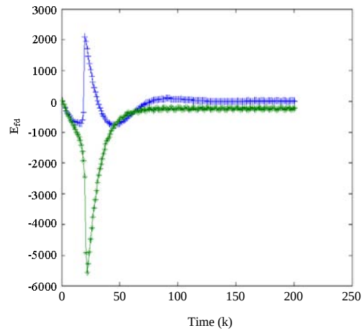
Fig. 18: The performance of E_{fd} ( \beta = 0.01 )
