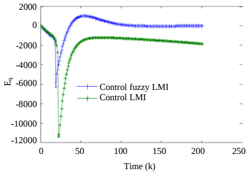
Fig. 10: The performance of E_d ( \beta = 0.01 )
