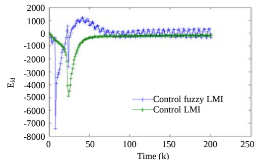
Fig. 26: The performance of E_B for \beta = 0.5 P, Q, X_e function
