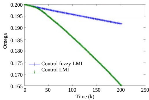
Fig. 16: The performance of \omega ( \beta = 0.01 )
