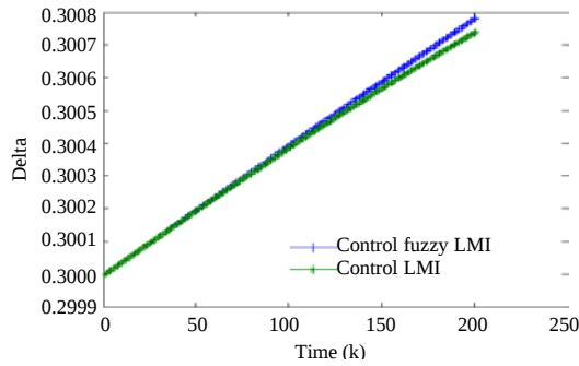
Fig. 15: The performance of \delta ( \beta = 0.01 )
