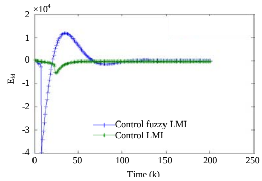
Fig. 24: The performance of E_{fd} for \beta = 0.5 ; P, Q, X_e constant
