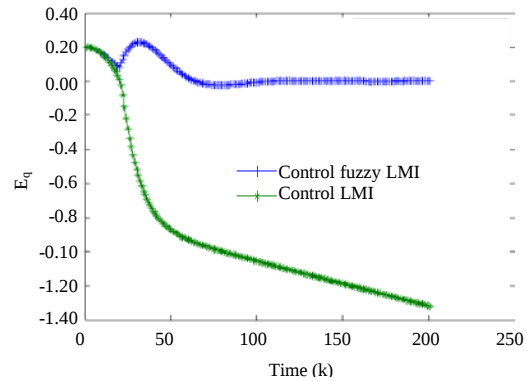
Fig. 17: The performance of E_q ( \beta = 0.01 )
