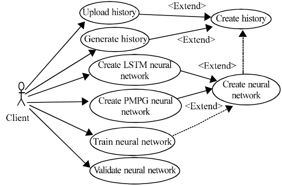
Fig. 4: Software characterization of PUs
