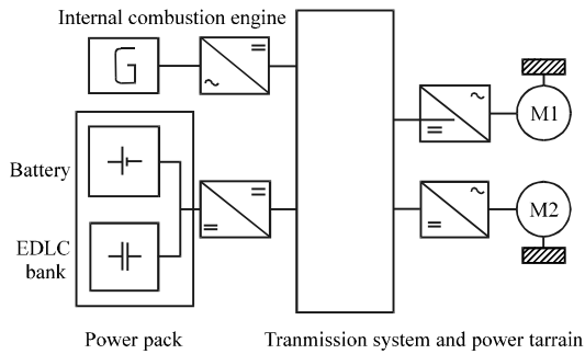
Fig. 4: Hybrid vehicle system
