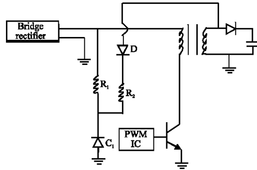
Fig. 1: Self-bias circuit
