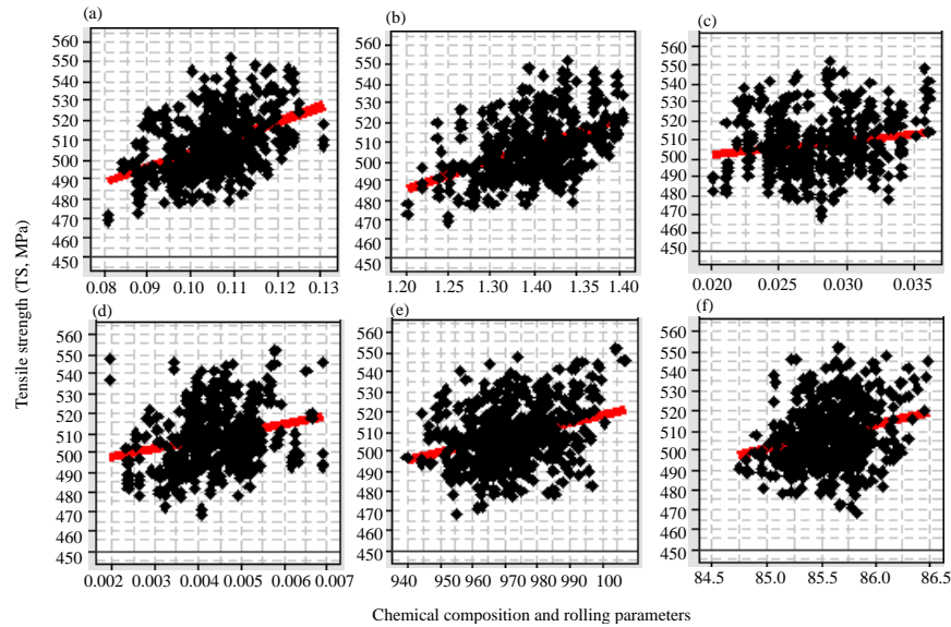
Fig. 4: Tensile strength vs. chemical compositions and process parameters for W200X46.1 steel beam (a) TS, Mpa°Carbon content (b) TS, Mpa°Magnesium content % (c) TS, Mpa°Niobium content % (d) TS, Mpa°Nitrogen content% (e) TS, Mpa°final temperature, Flange°C (f) TS, Mpa°Reduction, Flange % Scatterplot of TS, Mpa vs. chemical composition and rolling parameters (b) Chemical composition and rolling parameters
