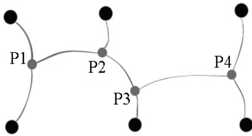
Fig. 3: Steiner's points P1-4
