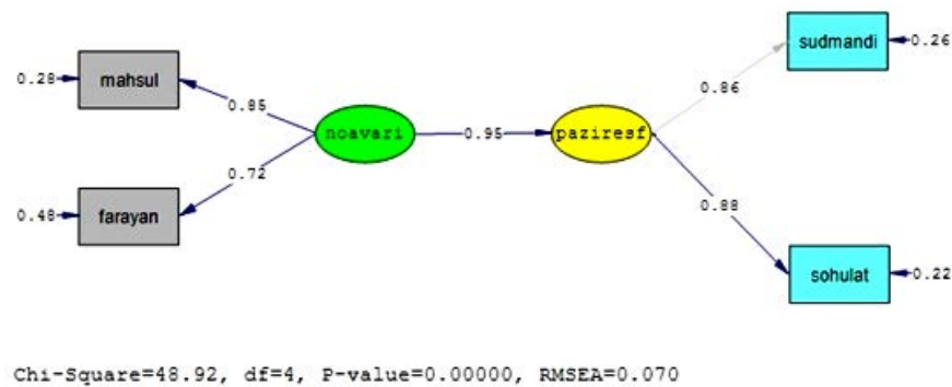
Fig. 6: Model in standard mode
