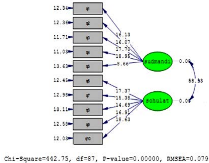
Fig. 2: Confirmatory factor analysis estimated first-ranging adoption of information technology in the standard model
