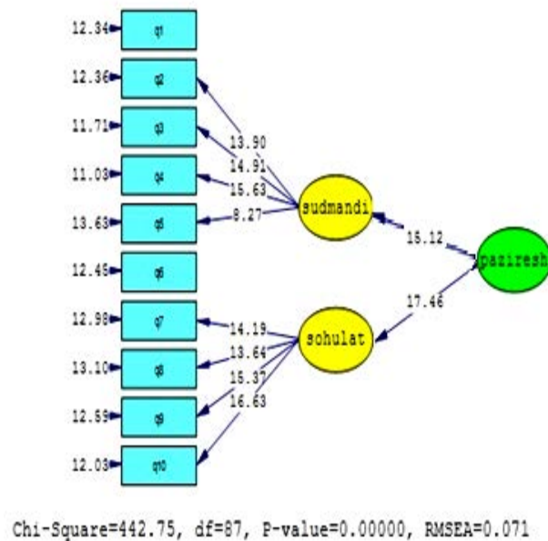
Fig. 3: Confirmatory factor analysis estimated second-ranging adoption of information technology in the standard model
