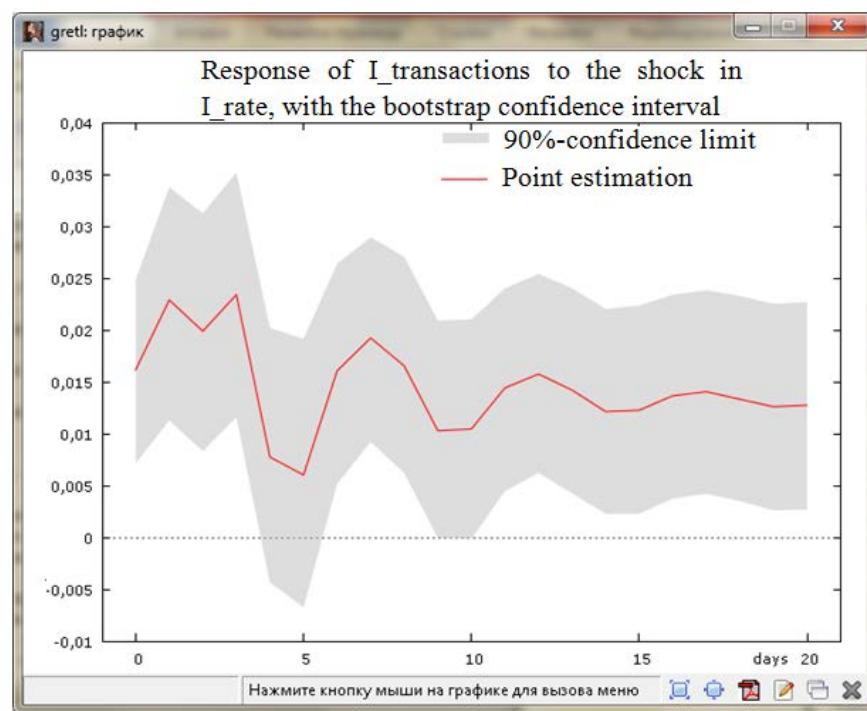
Fig. 7: Function of impulse response of in-transformed number of transactions and prices at Bitcoin. Response reaches 2.25% in the long-term period it equaled 1.25% from the initial value, moreover, lags that correspond to 4 and 5 response function is not significant
