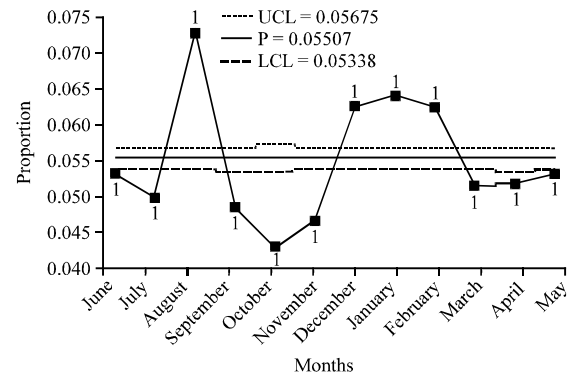
Fig. 5: P chart of total defect
