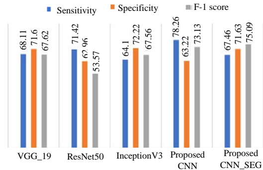
Fig. 7: Comparison of different networks with proposed CNN for classification of COVID-19
