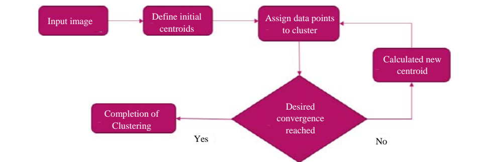
Fig. 2: Flow of k-means algorithm
